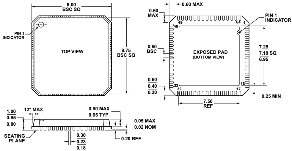
COMPLIANT TO JEDEC STANDARDS MO-220-VMMD-4 Figure 85. 64-Lead Lead Frame Chip Scale Package [LFCSP_VQ] 9 mm × 9 mm Body, Very Thin Quad (CP-64-3) Dimensions shown in millimeters
